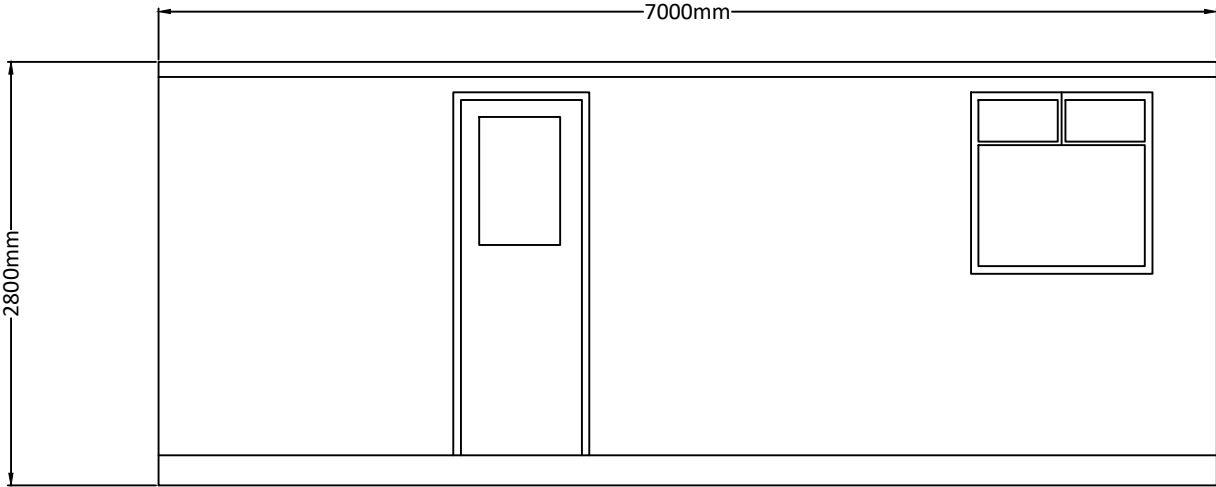
FRONT ELEVATION
